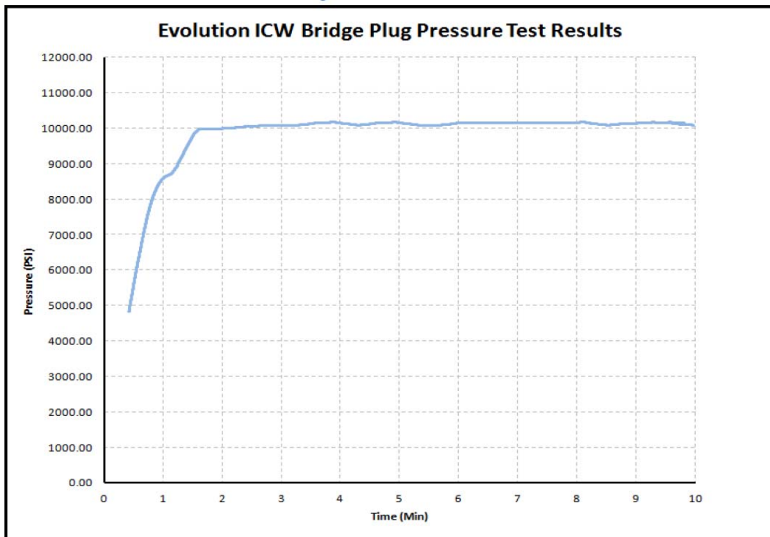
Figure 5 - Pressure Test Results
